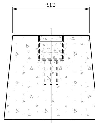
SECTION B
