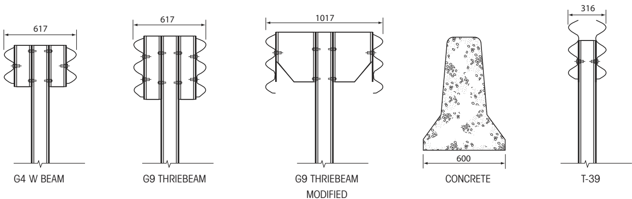
Figure 3: Barrier Comparisons – Median Applications
