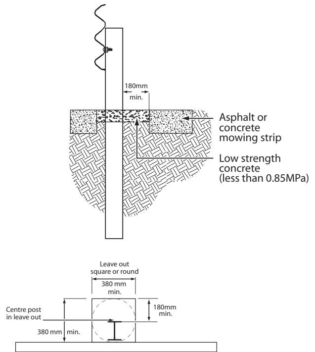
Figure 9: Post in Mowing Strips
