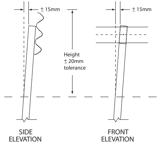
Figure 6: Post Tolerances - Side & Front View
