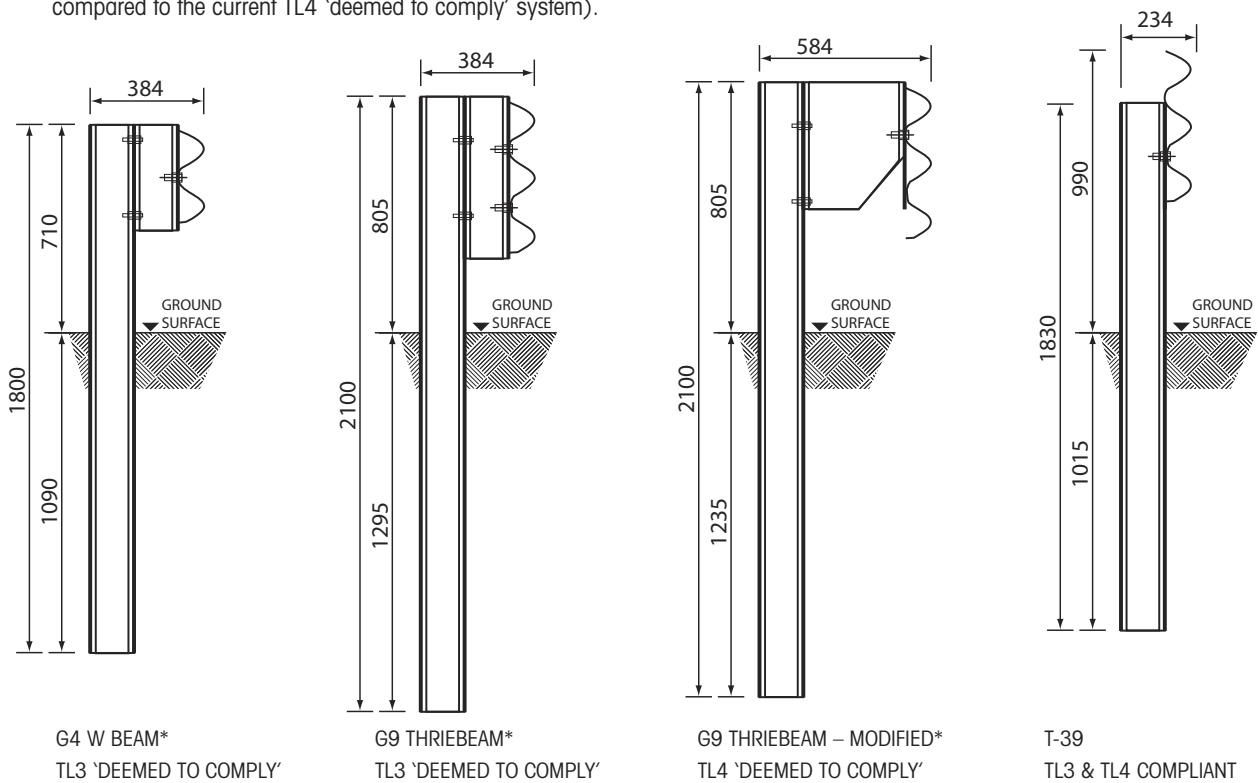
Figure 2: Barrier Comparisons – Verge Applications (*Denotes with C posts)
