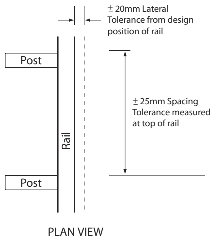
Figure 5: Post Tolerances Plan View
