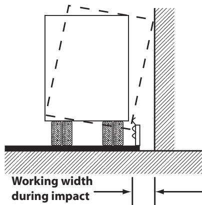
Figure 1: Working Width for TL4 Impact
